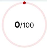
Performance score
